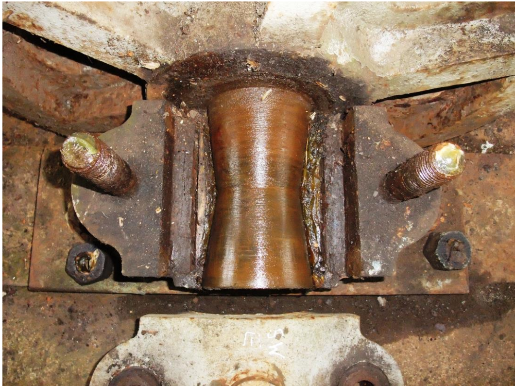
Plate 11 – SW Wheel – Inner bearing
