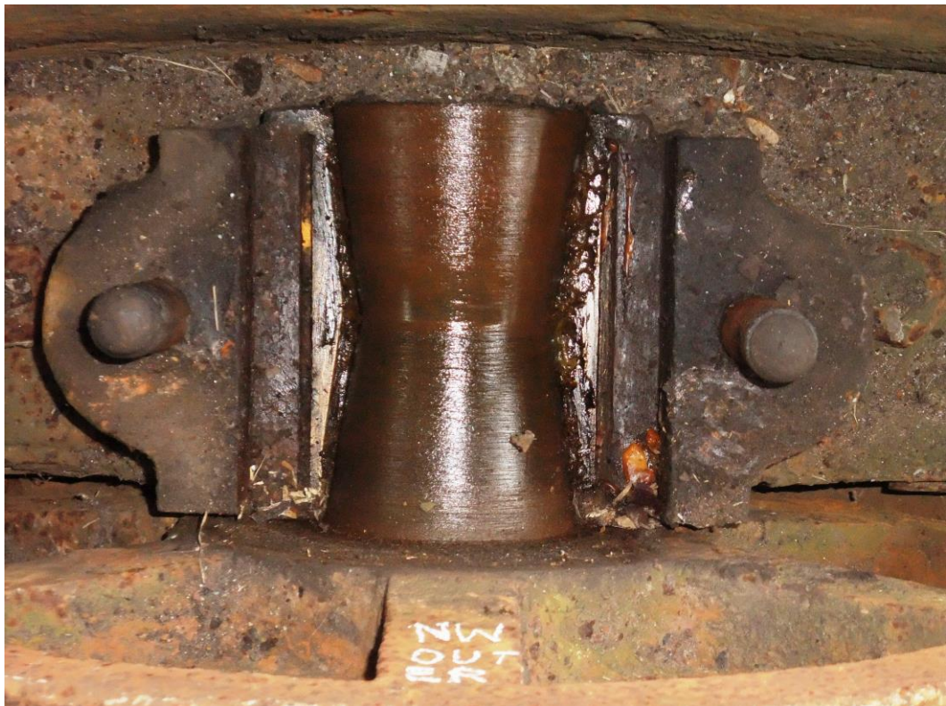
Plate 20 - NW Wheel – Outer bearing
