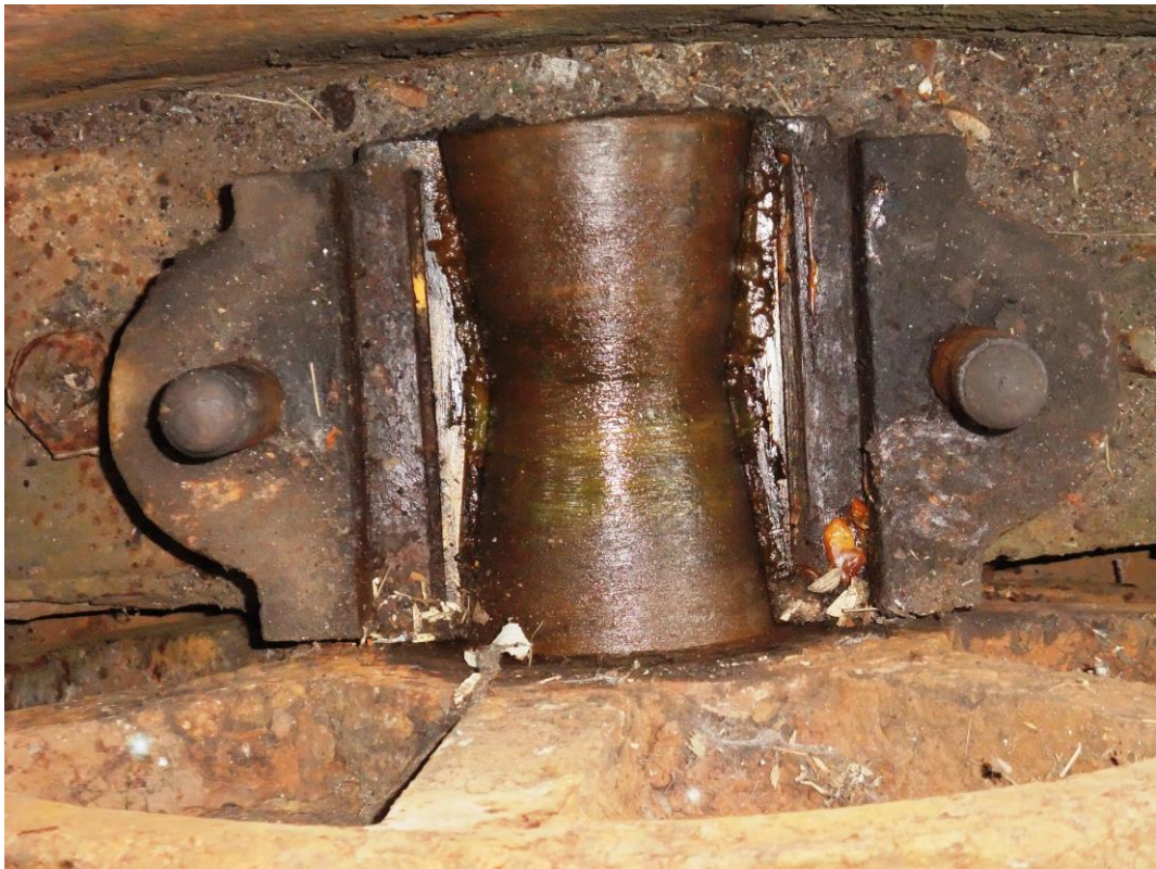
Plate 19 – NW Wheel – Outer bearing
